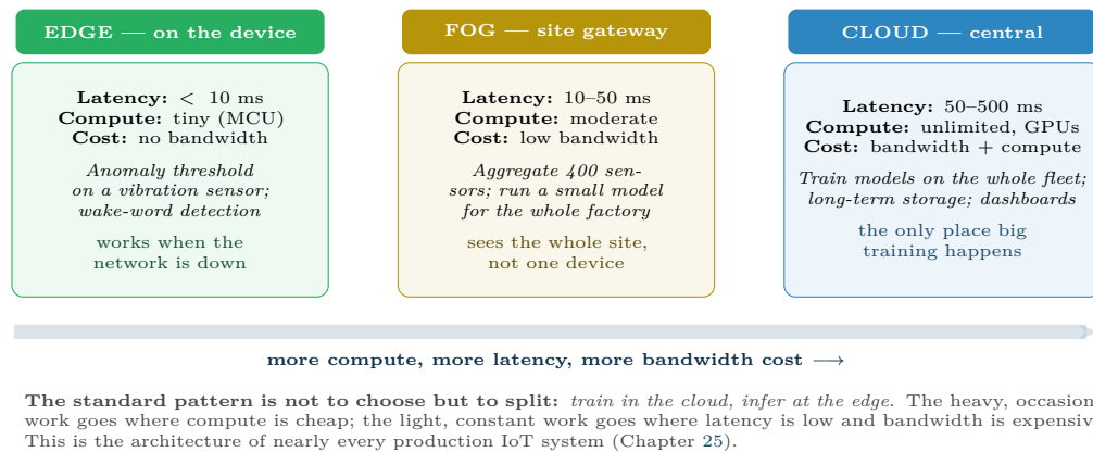
Figure 24.3: The three tiers. Placement is decided by the latency the decision requires and the bandwidth you can afford — not by where the computation is most convenient to write.
