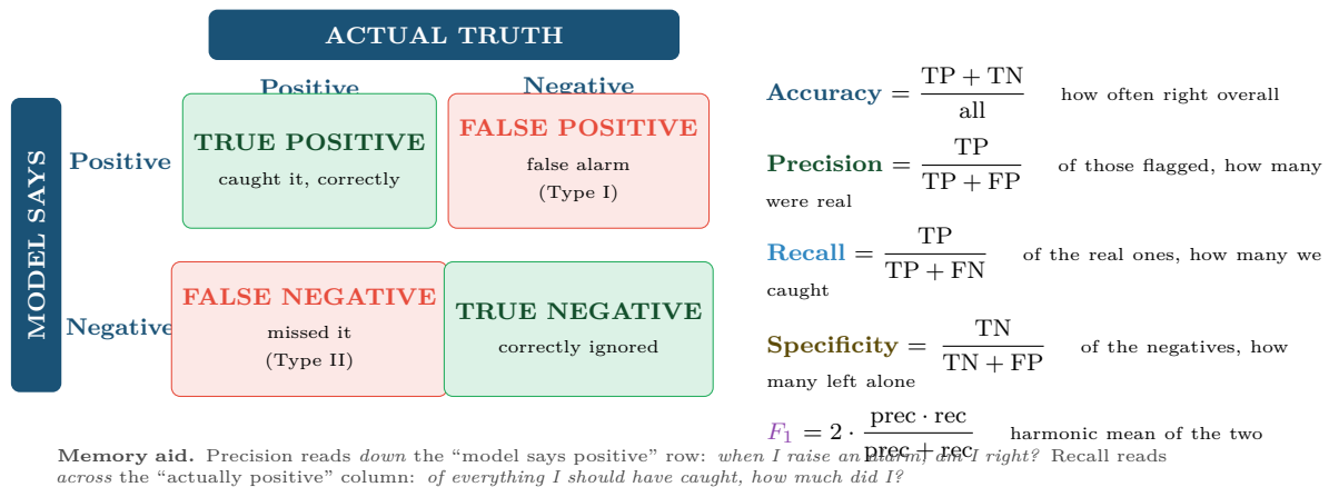
Figure 14.1: The confusion matrix and the five metrics derived from it. Learn which cells each metric uses; every question in this chapter reduces to that.
